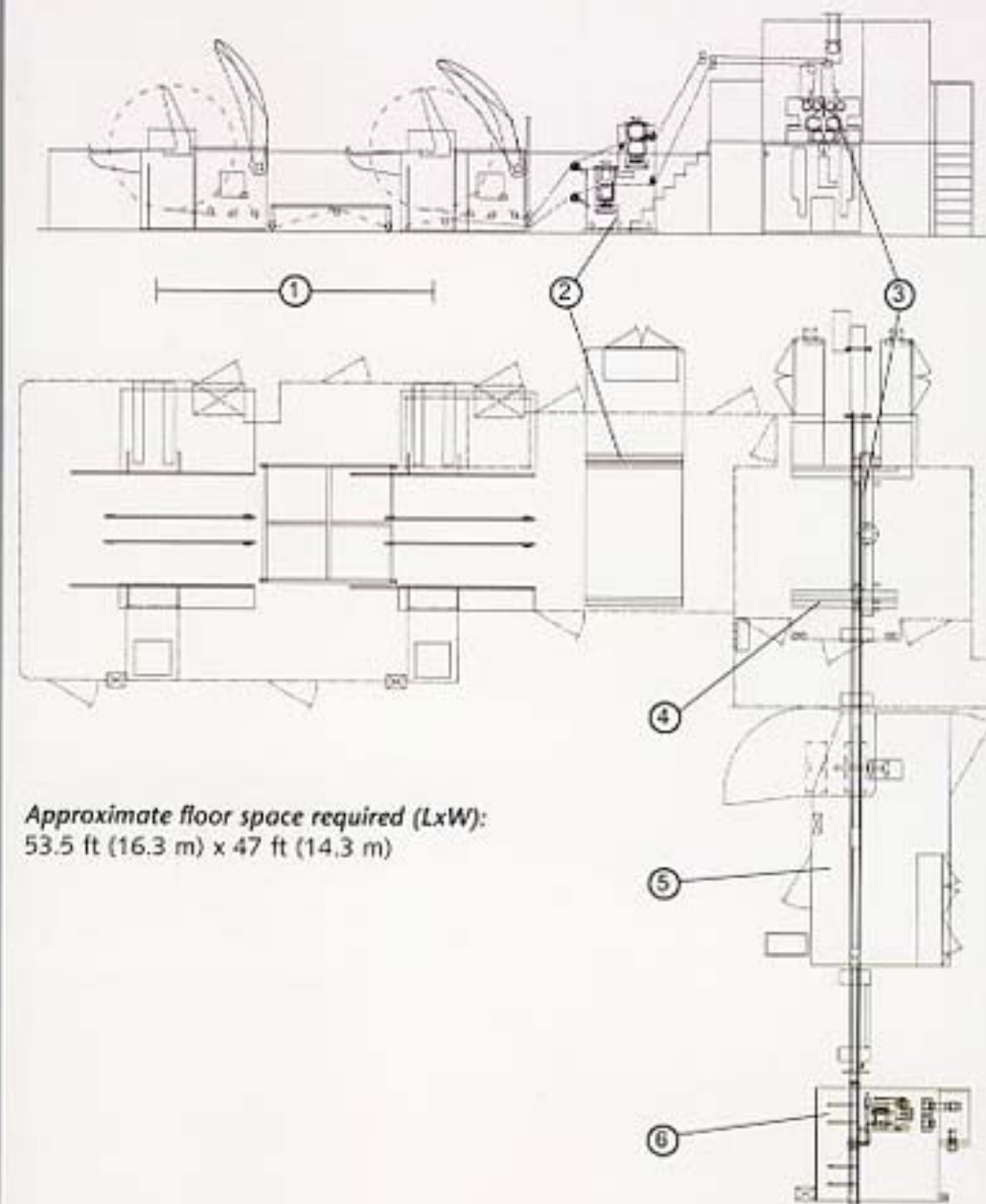
Dual-Station Calender Unit
