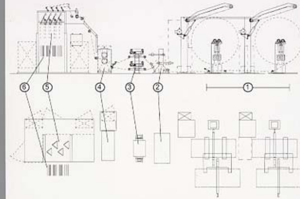
Self-Chucking Core-Ejecting Unwind Stand
